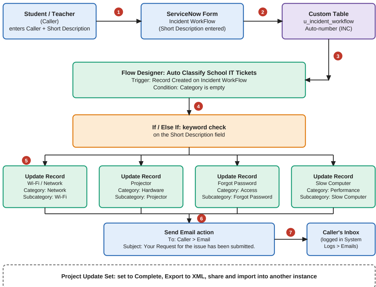
Figure 1: Architecture and data flow of the Auto Ticket Classification using Flow Designer solution
